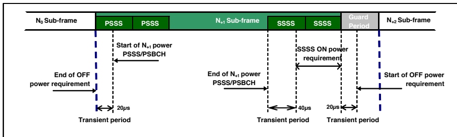
Figure 6.3.4D.3-2: PSSS/SSSS/PBCH time mask for extended CP transmission
