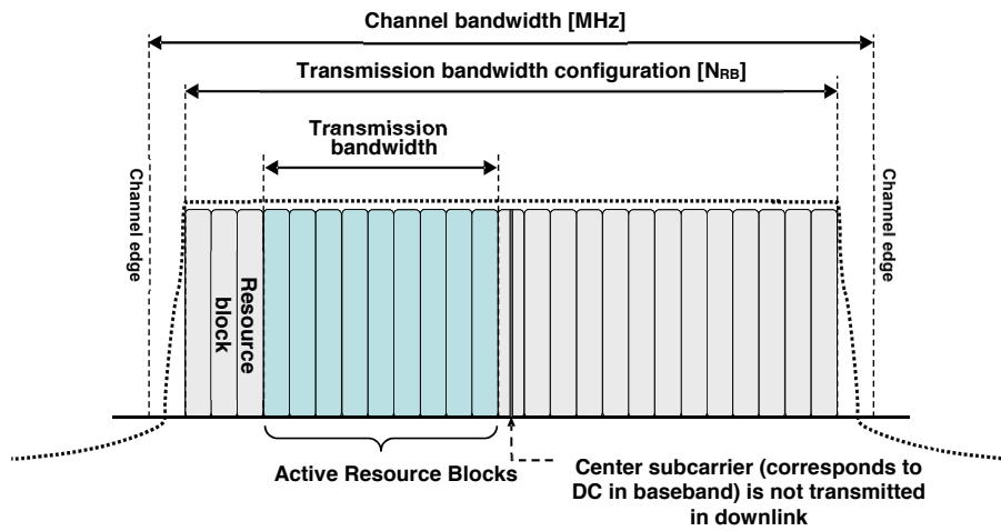
Figure 5.6-1: Definition of channel bandwidth and transmission bandwidth configuration for one E-UTRA carrier
