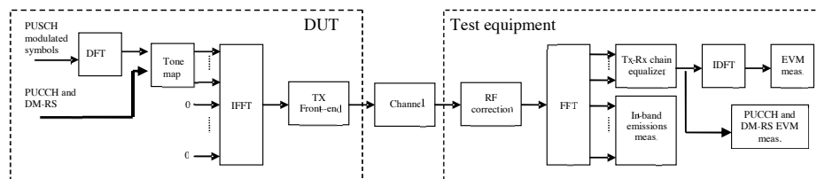
Figure F.1-1: EVM measurement points
