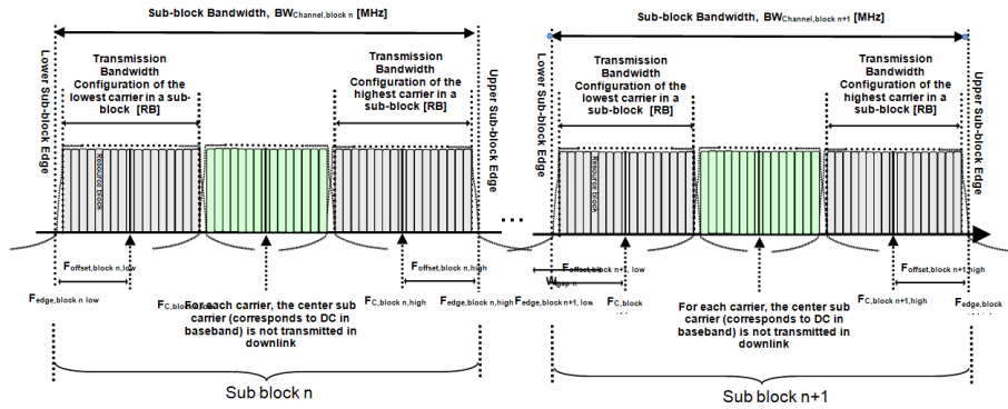
Figure 5.6A-2. Non-contiguous intraband CA terms and definitions
