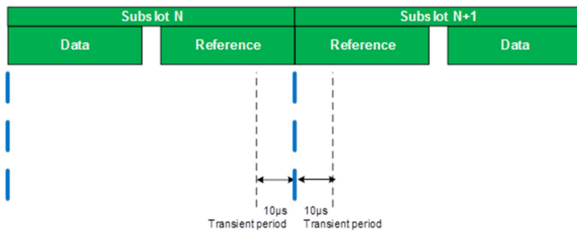
Figure 6.3.4.5-1: Transmission power template for subslot TT1 – transient period shared
