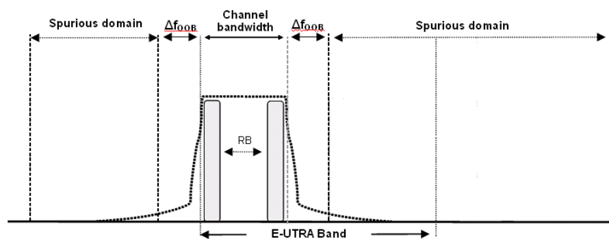
Figure 6.6-1: Transmitter RF spectrum
