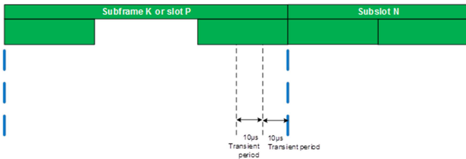
Figure 6.3.4.10-3: subframe TTI and subslot TTI boundary
