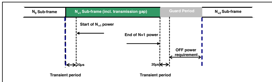
Figure 6.3.4D.1-1: PSDCH/PSCCH/PSSCH time mask
