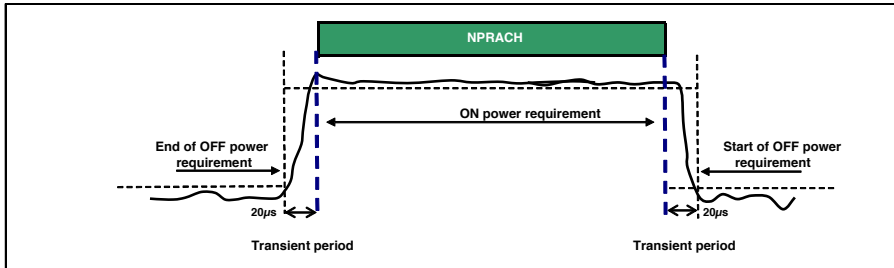
Figure 6.3.4F.2-1: NPRACH ON/OFF time mask
