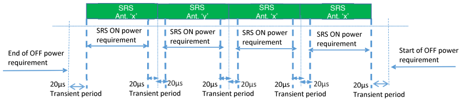
Figure 6.3.4.2.2-5: Time mask for SRS antenna switching
