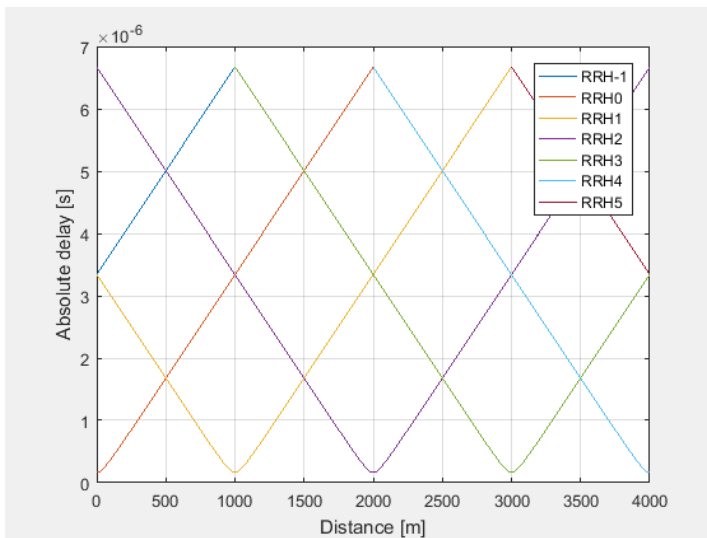
Figure B.3A-4 Relative delay trajectories
