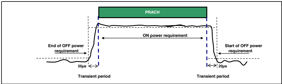
Figure 6.3.4.2-1: PRACH ON/OFF time mask
