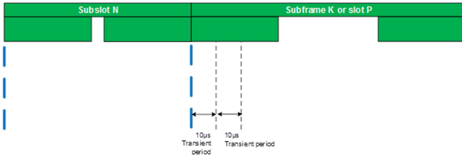
Figure 6.3.4.9-1: subslot TTI and subframe TTI boundary
