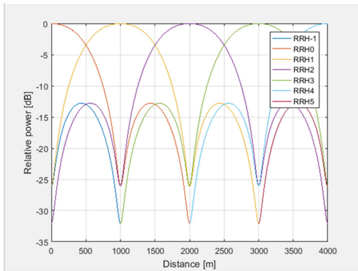
Figure B.3A-2 Relative power level trajectories
