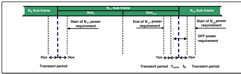
Figure 6.3.4.3-1A: Transmission power template when the bit in the associated DCI indicating the PUSCH ending symbol has value '1' for Frame Structure Type 3
