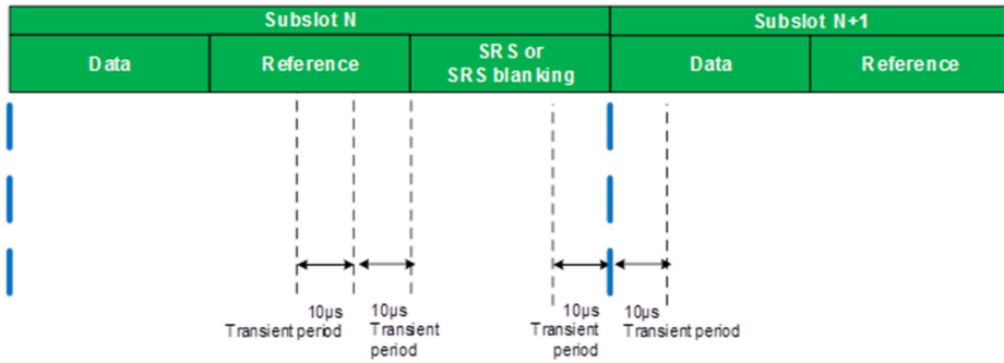
Figure 6.3.4.6-1: subslot PUSCH/SRS time mask when there is a Reference symbol before SRS (or SRS blanking) and data symbol after
