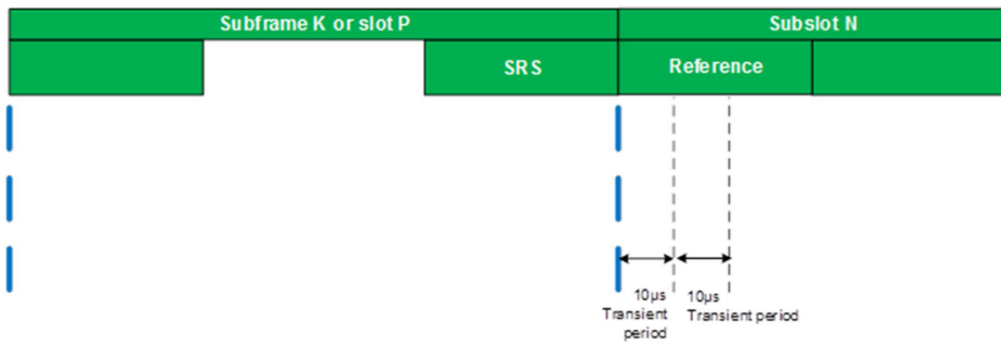
Figure 6.3.4.10-1: Subframe TTI and subslot TTI boundary with SRS in last subframe TTI symbol and Reference Symbol in first subslot TTI symbol
