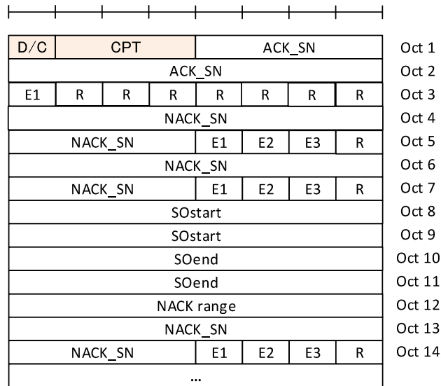
Figure 6.2.2.5-1: STATUS PDU with 12 bit SN
