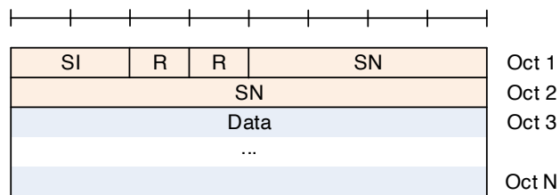
Figure 6.2.2.3-3: UMD PDU with 12 bit SN (No SO)
