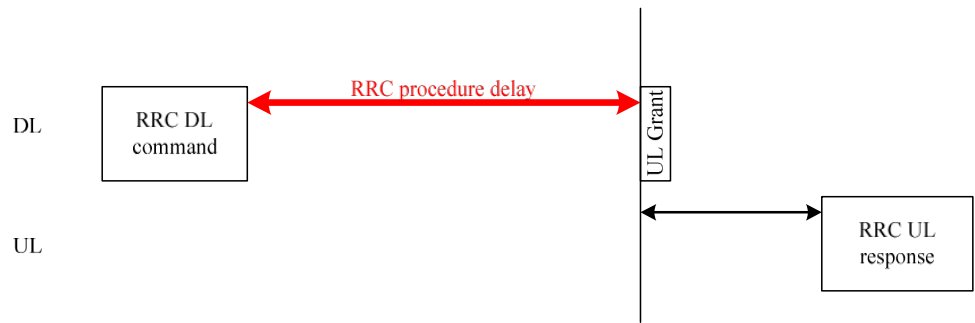
Figure 12.1-1: Illustration of RRC procedure delay
