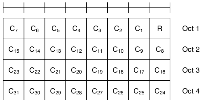
Figure 6.1.3.10-2: SCell Activation/Deactivation MAC CE of four octets
