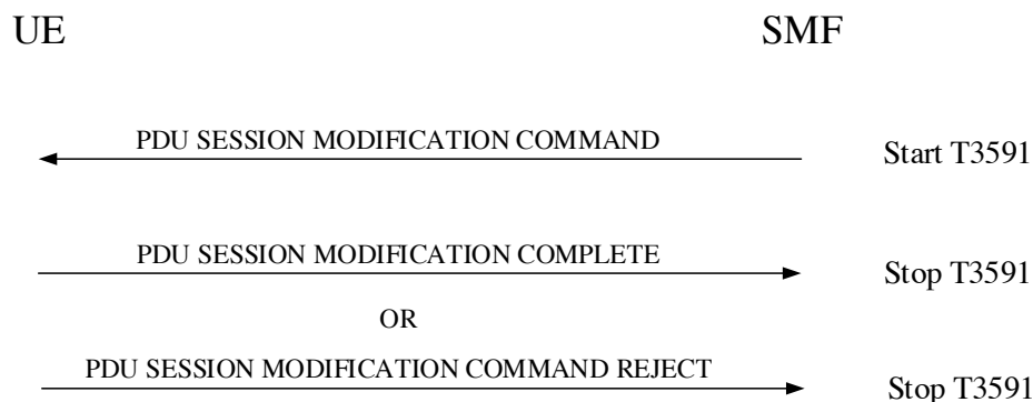
Figure 6.3.2.2.1: Network-requested PDU session modification procedure
