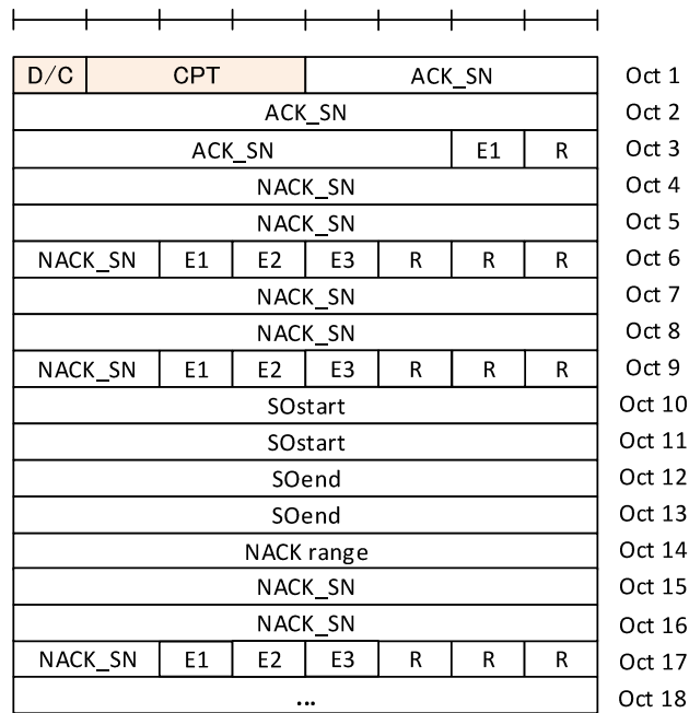
Figure 6.2.2.5-2: STATUS PDU with 18 bit SN
