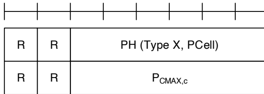
Figure 6.1.3.8-1: Single Entry PHR MAC CE
