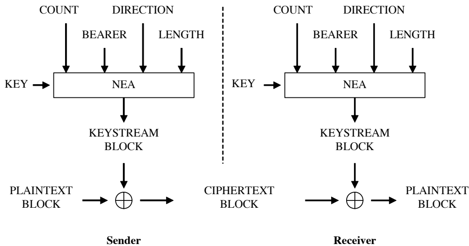
Figure D.2.1.1-1: Ciphering of data
