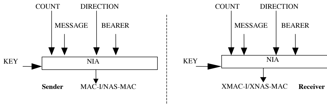
Figure D.3.1.1-1: Derivation of MAC-I/NAS-MAC (or XMAC-I/XNAS-MAC)
