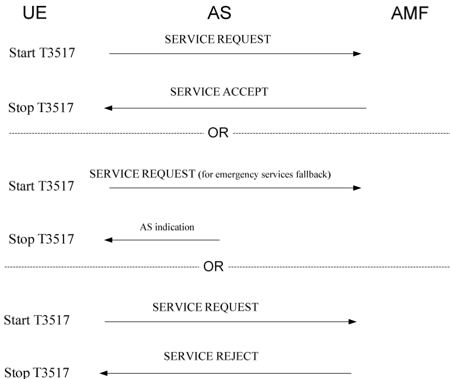
Figure 5.6.1.1.1: Service Request procedure
