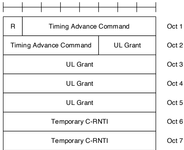
Figure 6.2.3-1: MAC RAR
