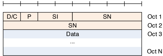
Figure 6.2.2.4-1: AMD PDU with 12 bit SN (No SO)
