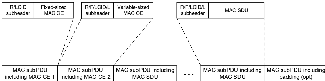
Figure 6.1.2-4: Example of a DL MAC PDU
