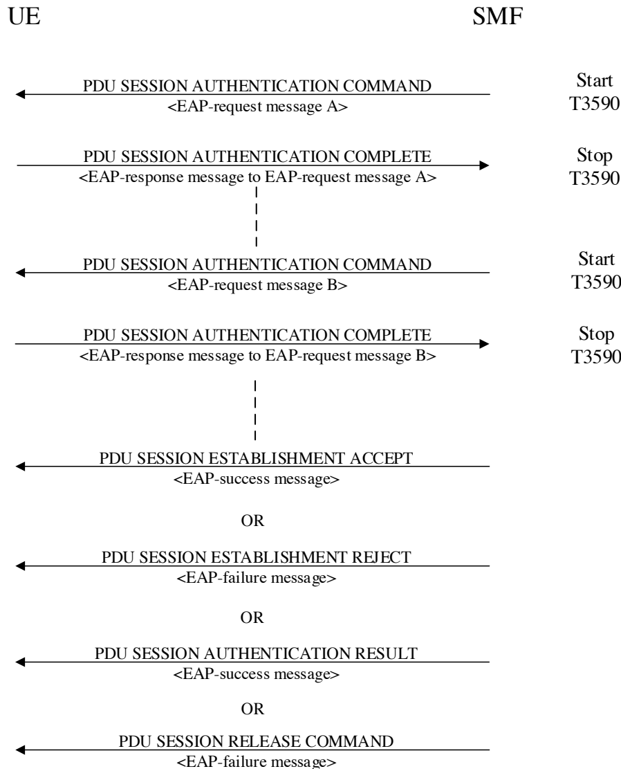
Figure 6.3.1.1: PDU session authentication and authorization procedure
