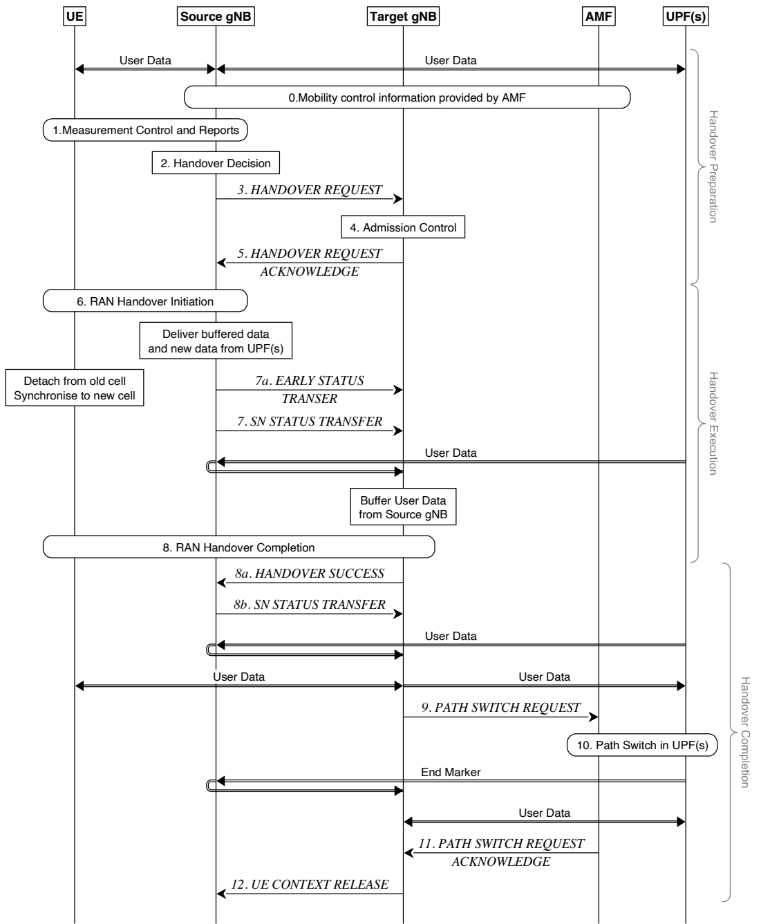
Figure 9.2.3.2.1-1: Intra-AMF/UPF Handover
