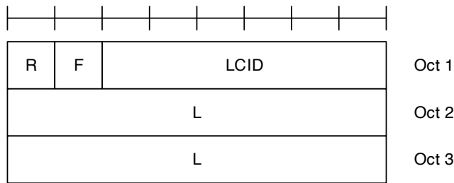
Figure 6.1.2-2: R/F/LCID/L MAC subheader with 16-bit L field
