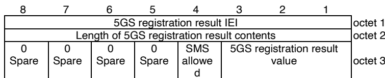
Figure 9.11.3.6.1: 5GS registration result information element
