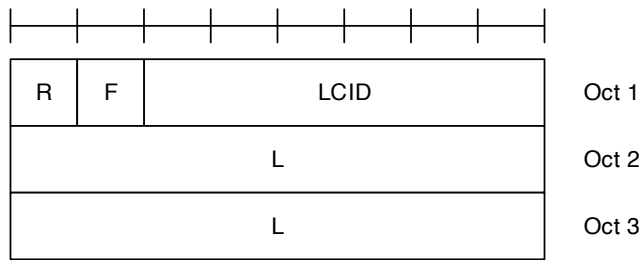
Figure 6.1.2-2: R/F/LCID/L MAC subheader with 16-bit L field
