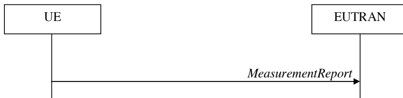
Figure 5.5.5.1-1: Measurement reporting
