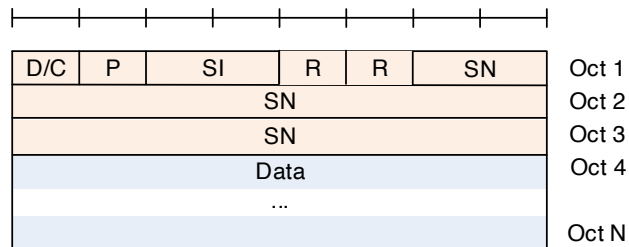
Figure 6.2.2.4-2: AMD PDU with 18 bit SN (No SO)
