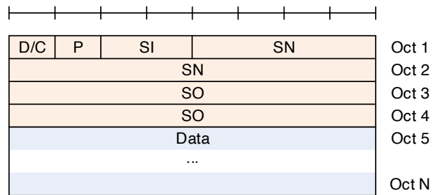
Figure 6.2.2.4-3: AMD PDU with 12 bit SN with SO
