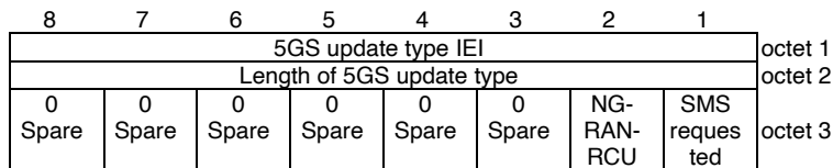
Figure 9.11.3.9A.1: 5GS update type information element
