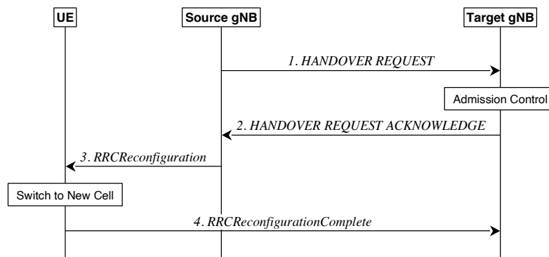
Figure 9.2.3.1-1: Inter-gNB handover procedures
