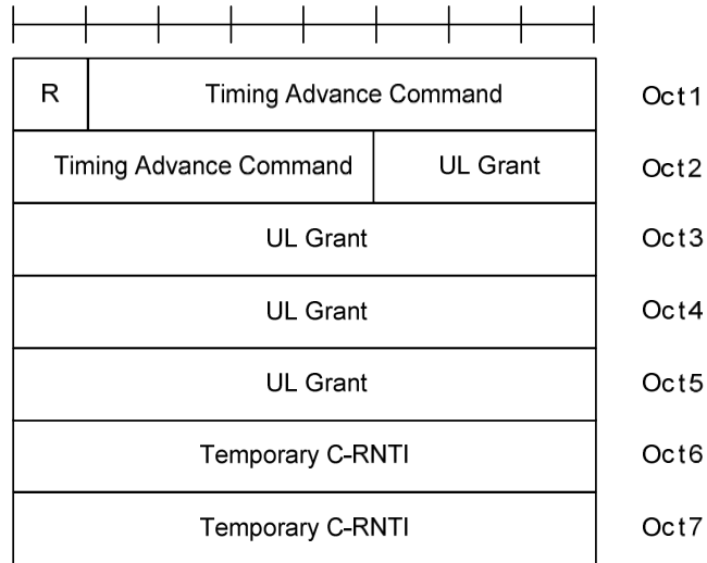
Figure 6.2.3-1: MAC RAR
