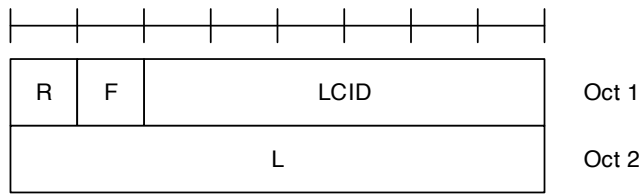
Figure 6.1.2-1: R/F/LCID/L MAC subheader with 8-bit L field
