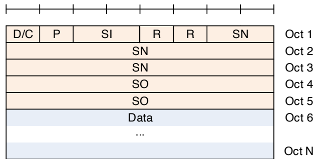
Figure 6.2.2.4-4: AMD PDU with 18 bit SN with SO
