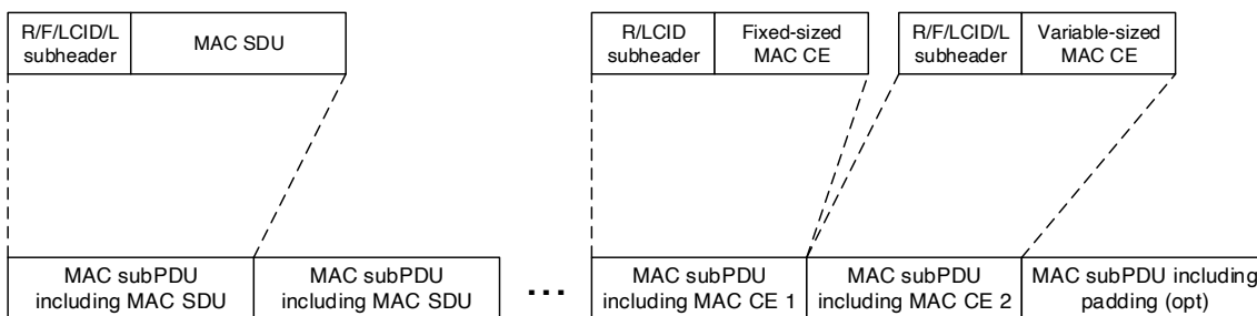
Figure 6.1.2-5: Example of a UL MAC PDU
