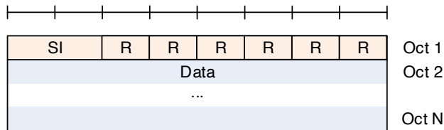
Figure 6.2.2.3-1: UMD PDU containing a complete RLC SDU
