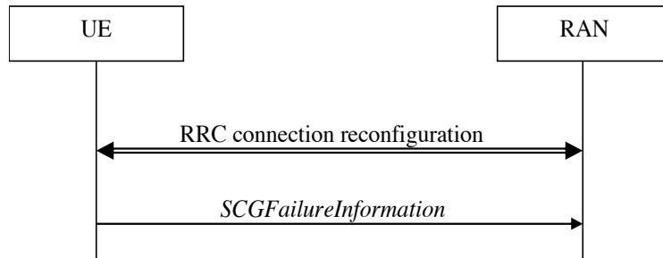
Figure 5.7.3.1-1: SCG failure information
