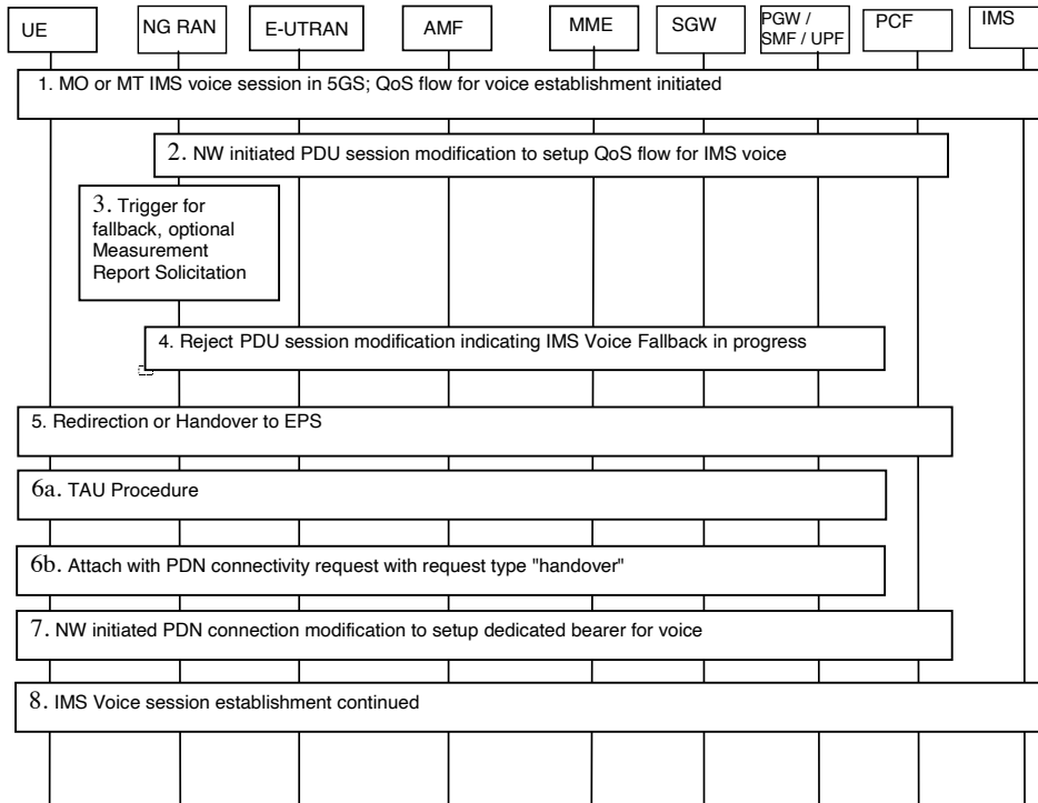
Figure 4.13.6.1-1: EPS Fallback for IMS voice
