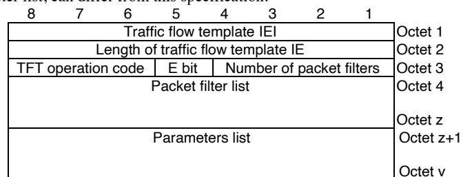
Figure 10.5.144/3GPP TS 24.008: Traffic flow template information element
