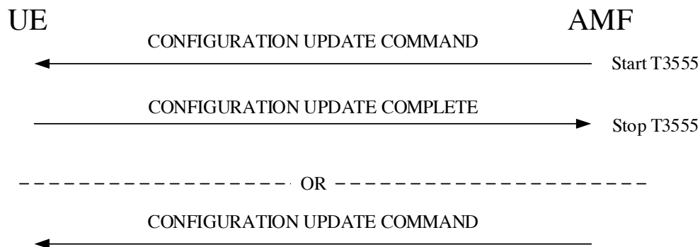
Figure 5.4.4.1.1: Generic UE configuration update procedure
