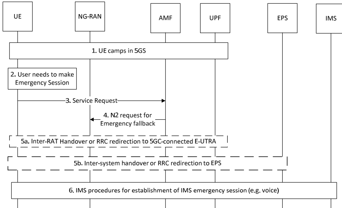
Figure 4.13.4.2-1: Emergency Services Fallback
