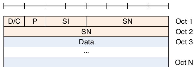
Figure 6.2.2.4-1: AMD PDU with 12 bit SN (No SO)
