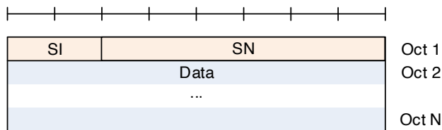
Figure 6.2.2.3-2: UMD PDU with 6 bit SN (No SO)
