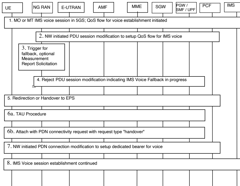
Figure 4.13.6.1-1: EPS Fallback for IMS voice
